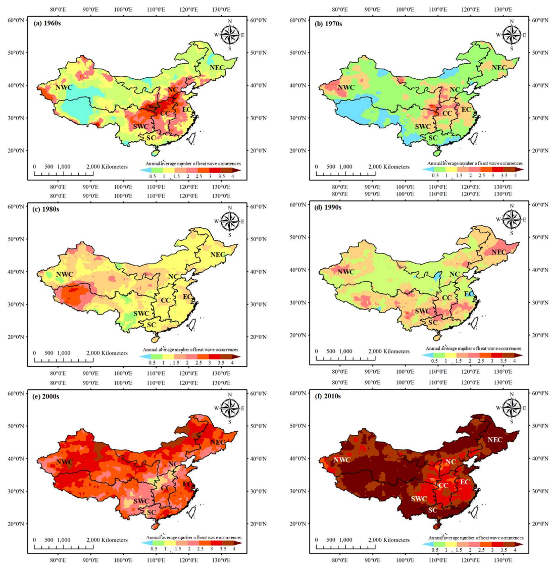
Figure 4. Spatial distribution of annual average number of heat wave occurrences at decadal level: (a) 1960s, (b) 1970s, (c) 1980s, (d) 1990s, (e) 2000s, and (f) 2010s.
