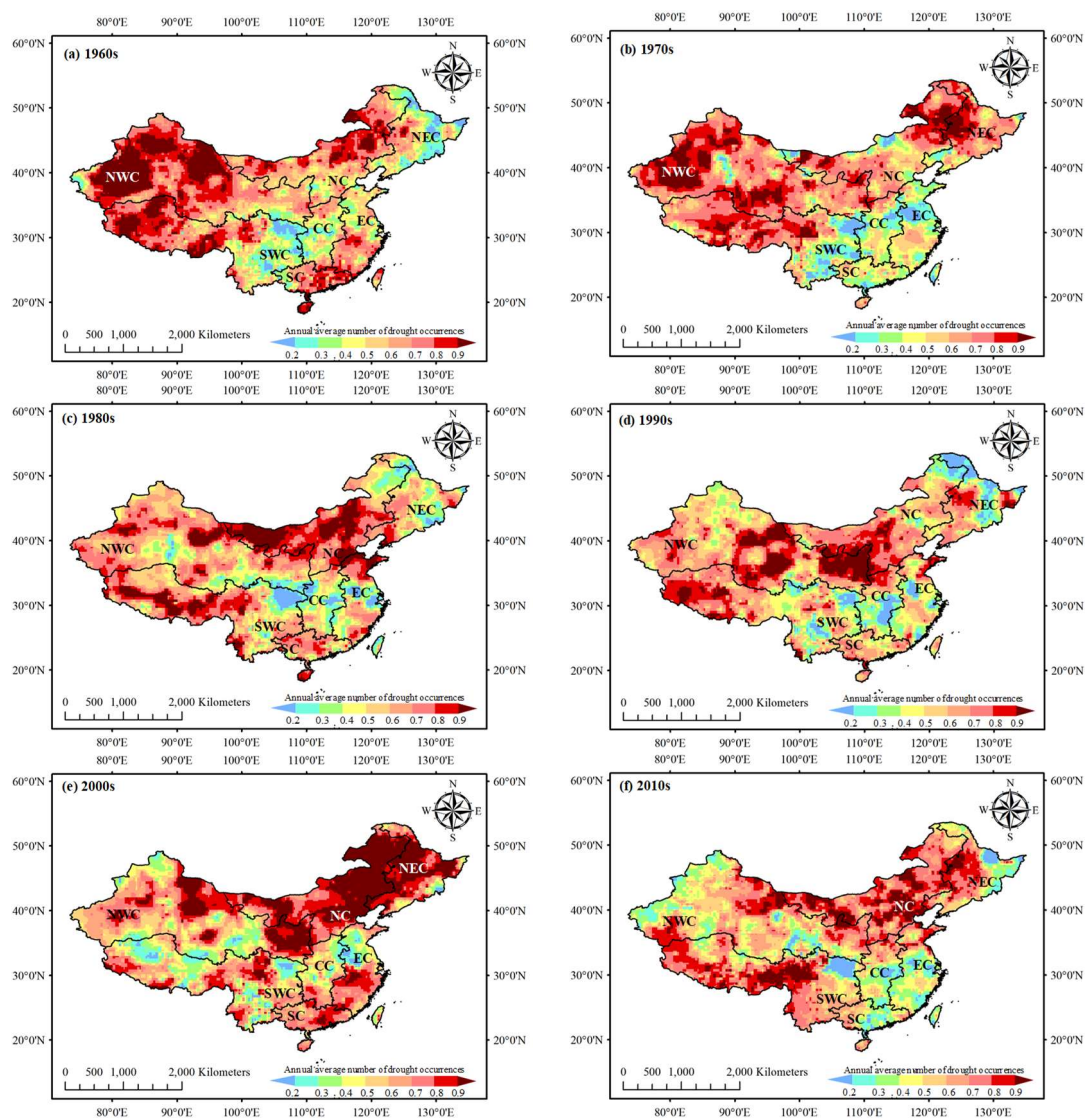
Figure 2. Spatial distribution of annual average number of drought occurrences at decadal level: (a) 1960s, (b) 1970s, (c) 1980s, (d) 1990s, (e) 2000s, and (f) 2010s.
