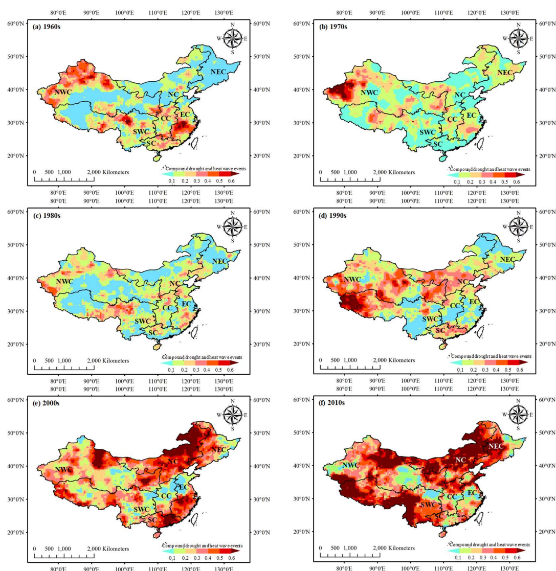
Figure 6. Spatial distribution of annual average number of compound drought and heat wave occurrences at decadal level: (a) 1960s, (b) 1970s, (c) 1980s, (d) 1990s, (e) 2000s, and (f) 2010s.
