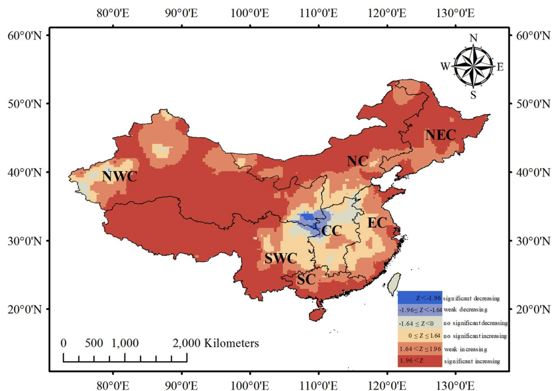
Figure 5. Spatial structure of daily maximum temperature trends from the 1960s to 2010s.
