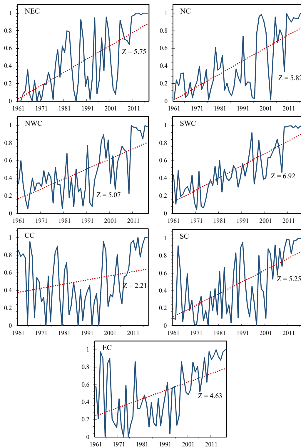
Figure 7. Percentage of compound droughts and heat waves to droughts for the seven regions from 1961–2017.
