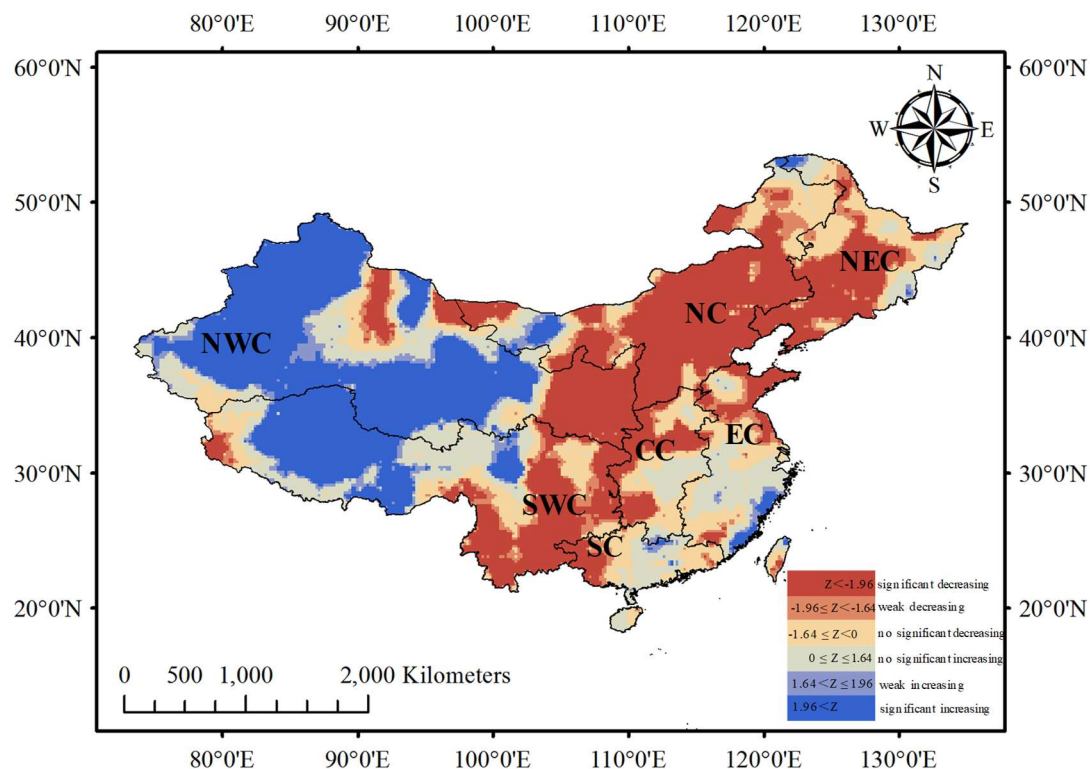
Figure 3. Spatial structure of sc_PDSI trends during 1960s–2010s.
